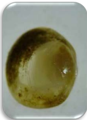
Procladius sp.
