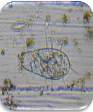
Euglyphasp.
