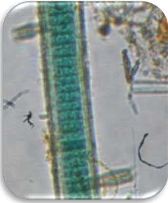
Stauroneis sp.
