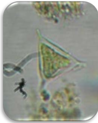
Tetradon sp.
