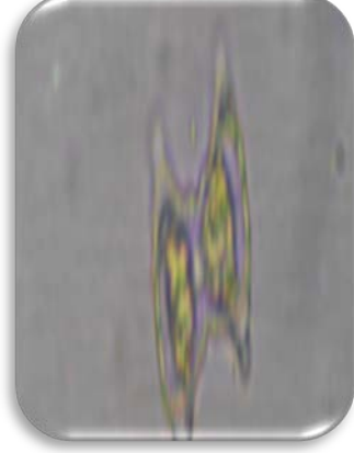
Tetradon sp.
