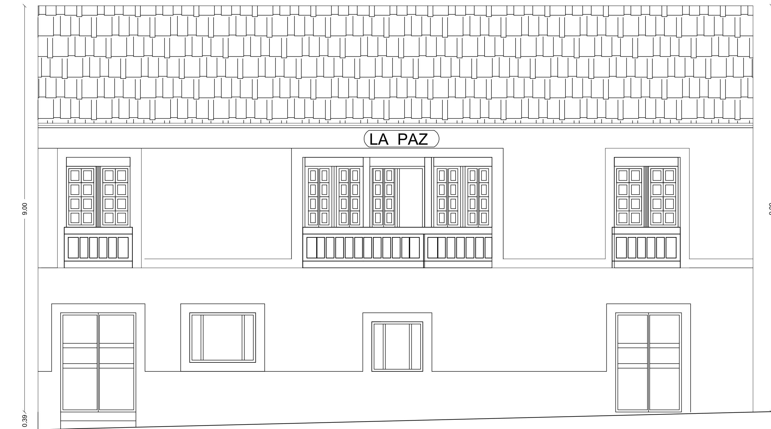
FACHADA PRINCIPAL Escala _____1:50
