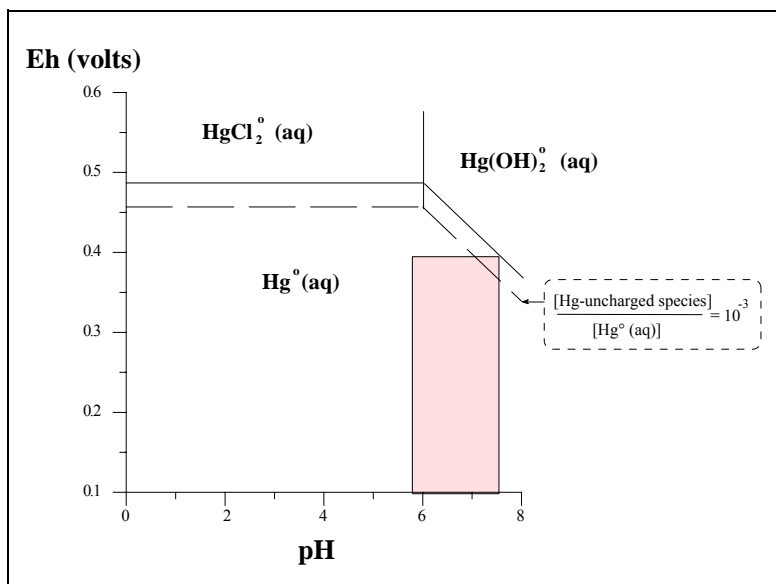
Fig. 1.7. Equilibrium boundaries of \text{Hg}^\circ (aq) and Hg-inorganic complexes
