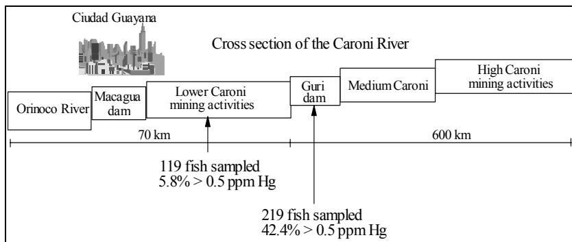
Fig. 1.13. Comparison of Hg levels in fish from Lower Caroni River and Guri Reservoir in Venezuela (Veiga, 1997)
