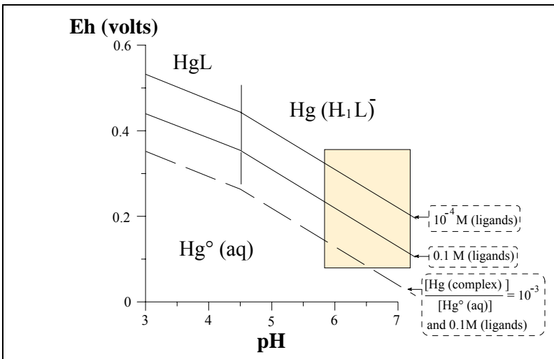
Fig. 1.8. Equilibrium boundaries of Hg^{\circ}(aq) and Hg-organic complexes : Typical conditions of Eh and pH of Amazonian sediments.
