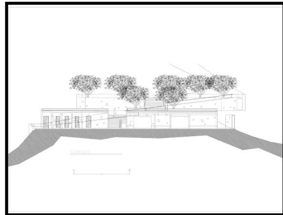
Figura 51. Fachada www.archdaily.co/co/02-59882/mirador-vina-sena-german-del-sol
