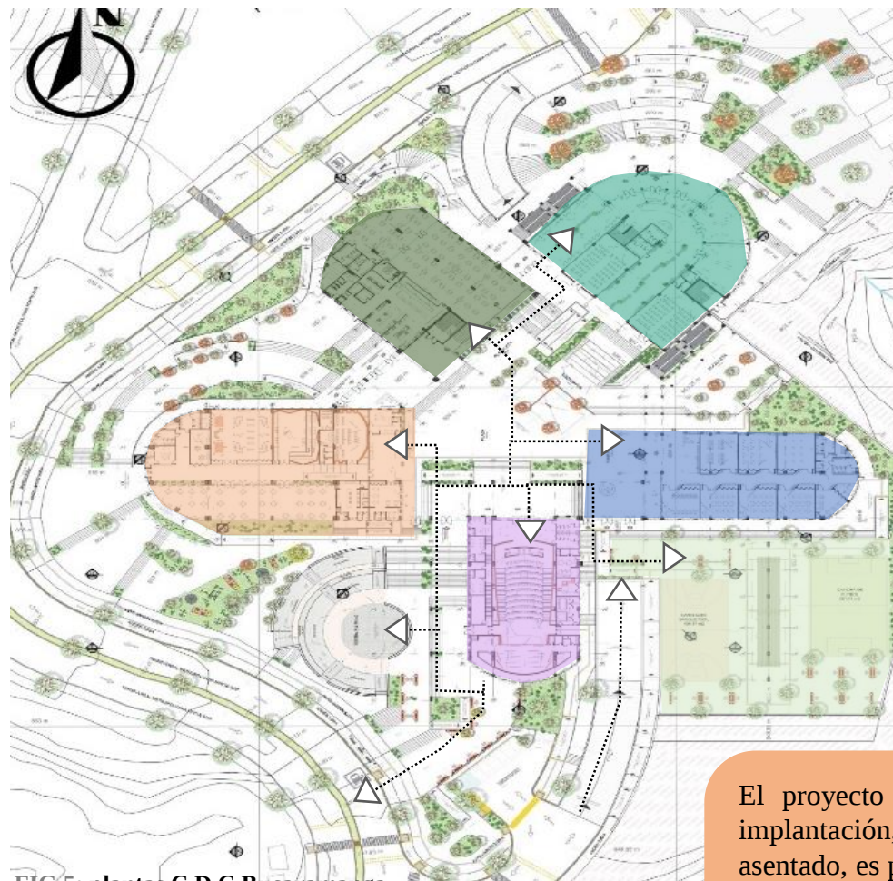
FIG 5: plantas C.D.C Bucaramanga
