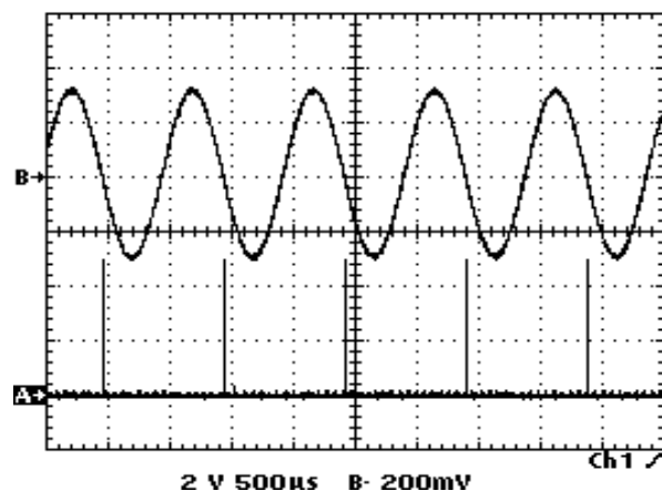
Figure 7-34. Waveform - A8/A24 Monitor CCA TP9 and TP8
