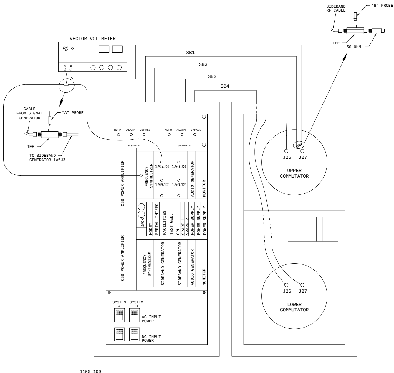
Figure 9-13. Test Equipment Setup for Sideband Cable Calibration
