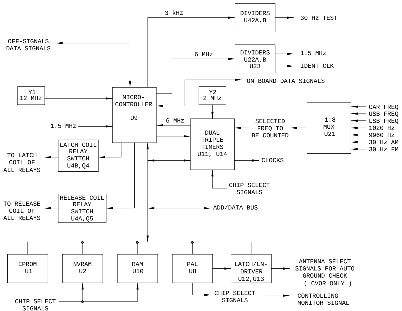
Figure 2-38. Monitor CCA, Block Diagram (sheet 1)
