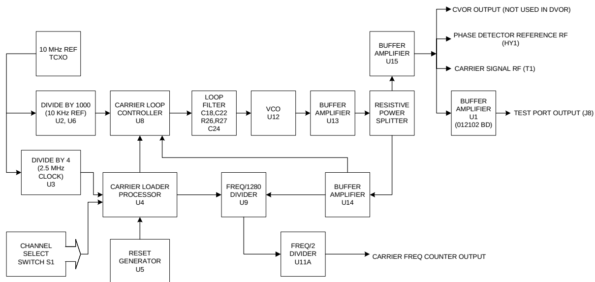
Figure 2-4. Carrier RF Generation Loop
