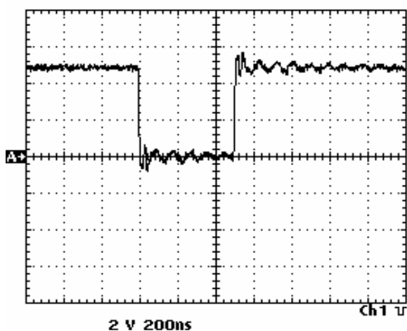
Figure 7-47. Waveform - A8/A24 TP16 300 Hz Clock Pulse
