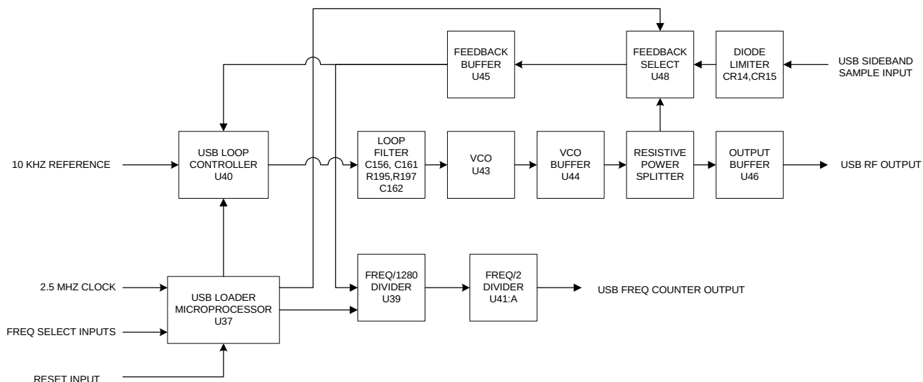
Figure 2-6 Upper Sideband RF Generation Loop
