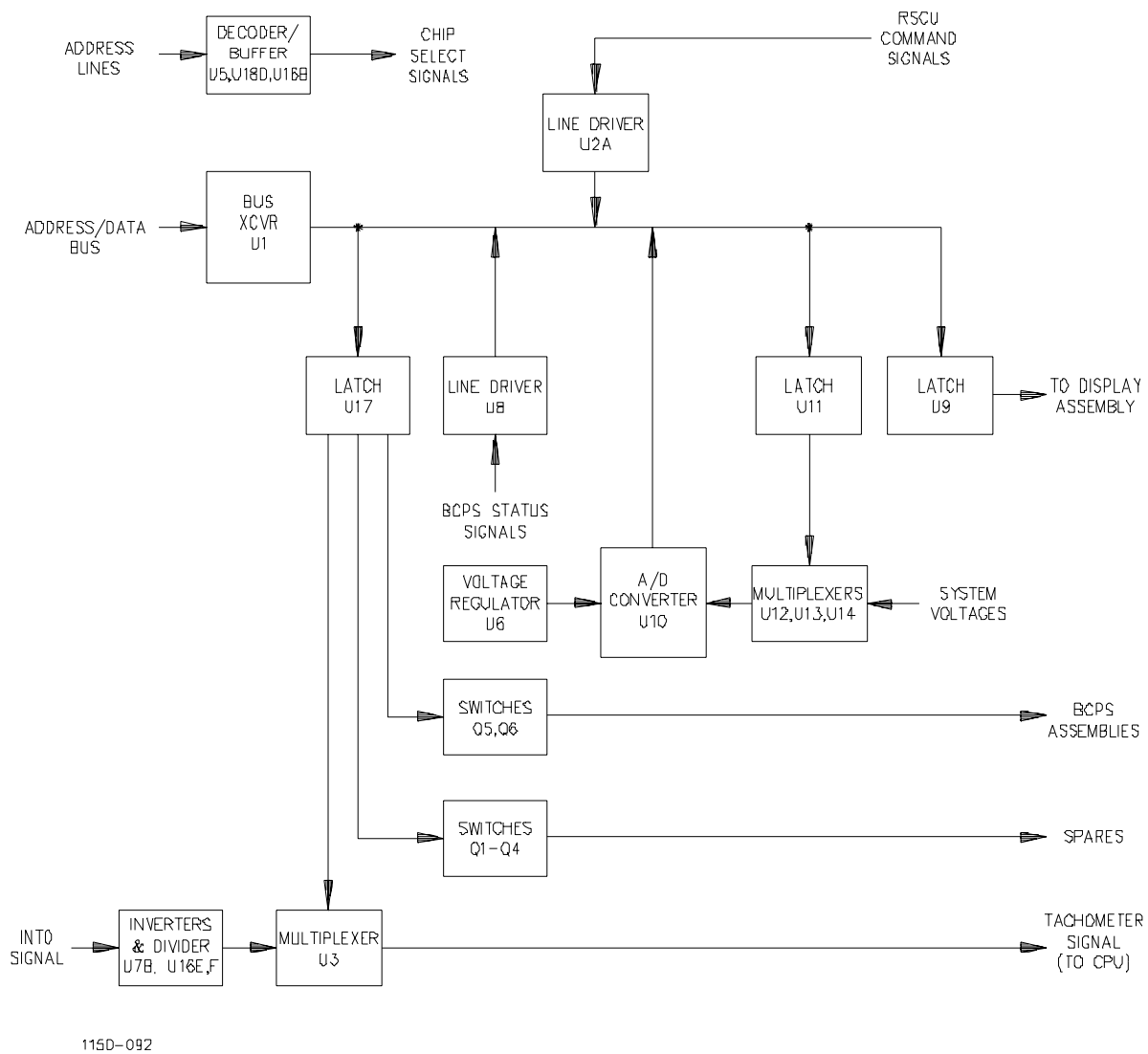
Figure 2-29. Facilities CCA Block Diagram
