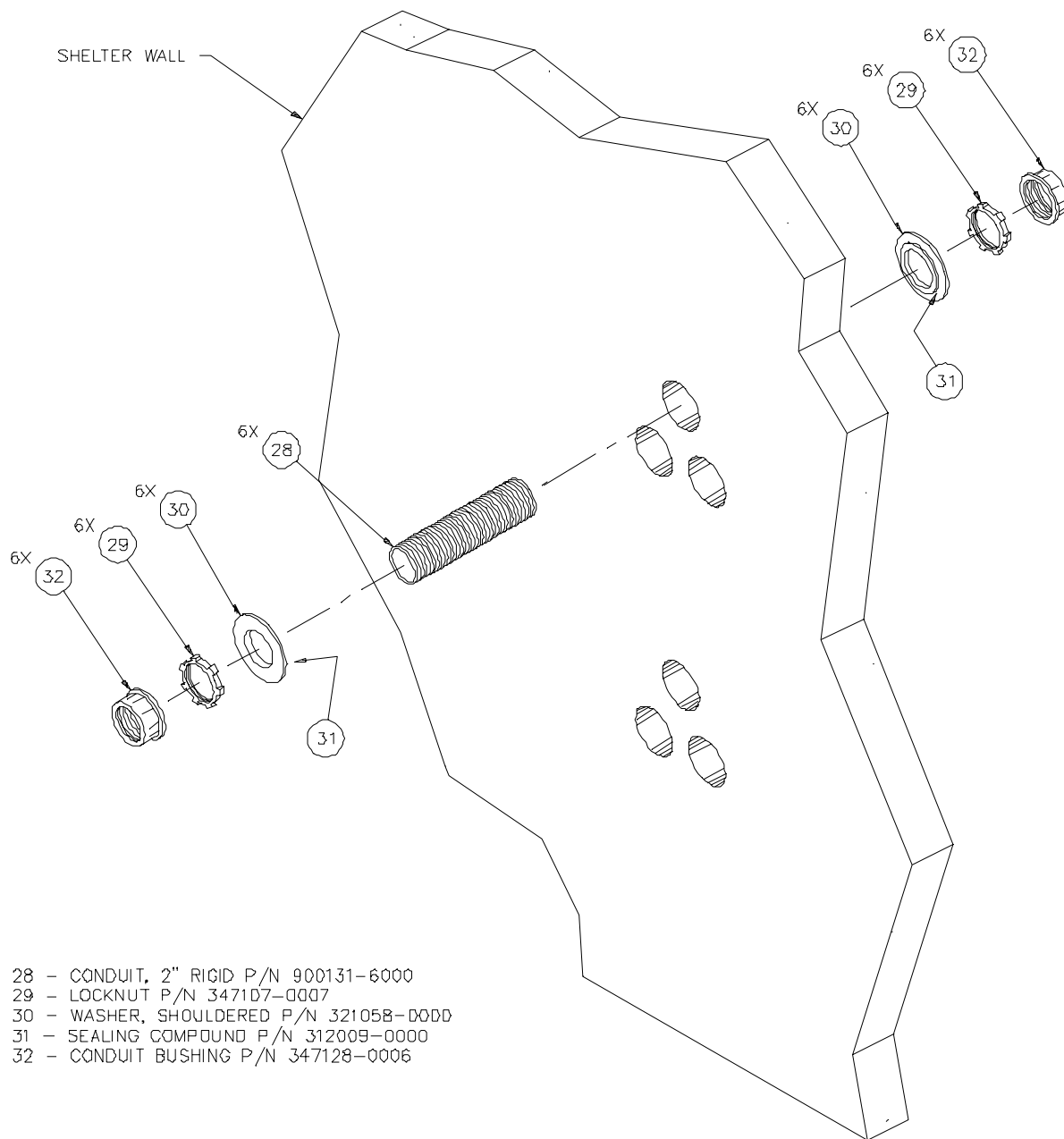
Figure 9-3. Exterior Cable Entrance Installation
