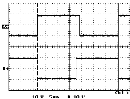
Figure 7-43. Waveform - A8/A24 TP15 and TP7 (0 Degrees)
