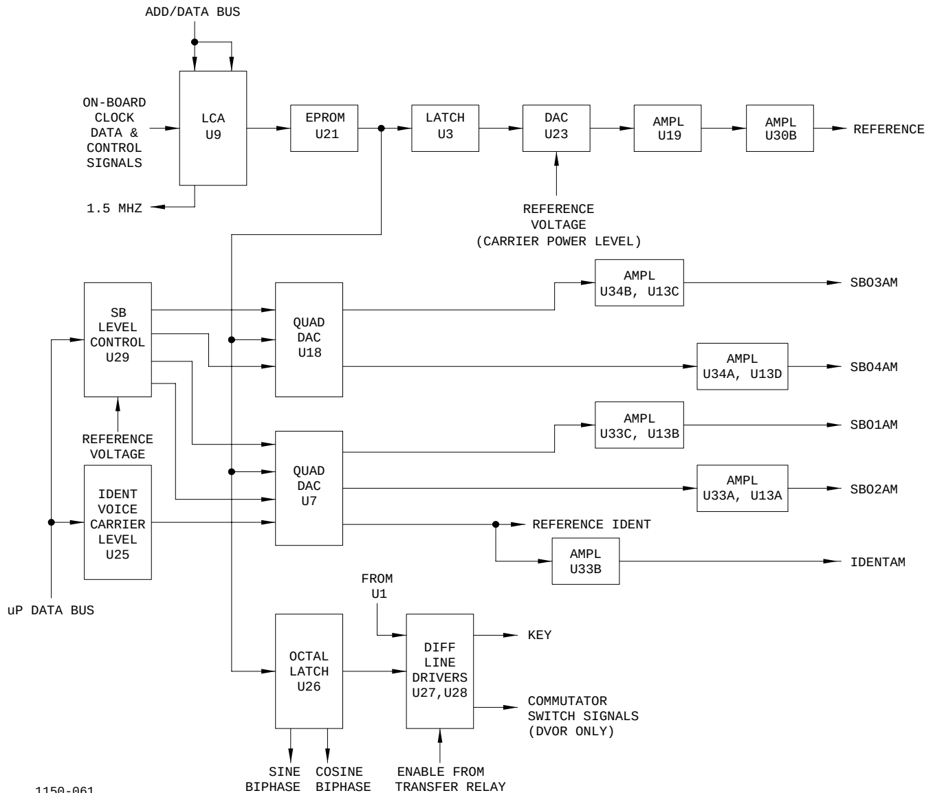
Figure 2-9. Audio Generator CCA Block Diagram
