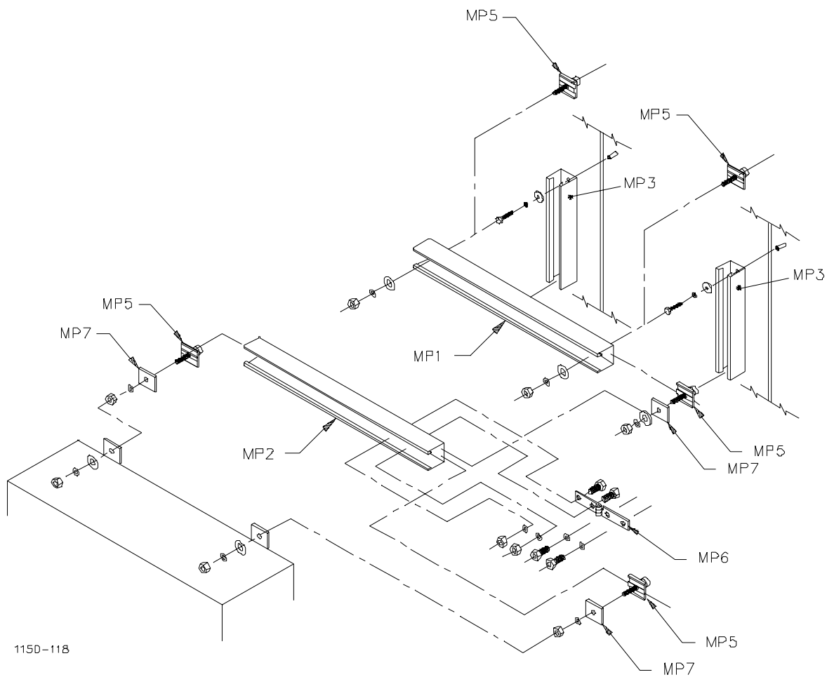
Figure 9-6. Transmitter Cabinet to Shelter Wall Installation Diagram
