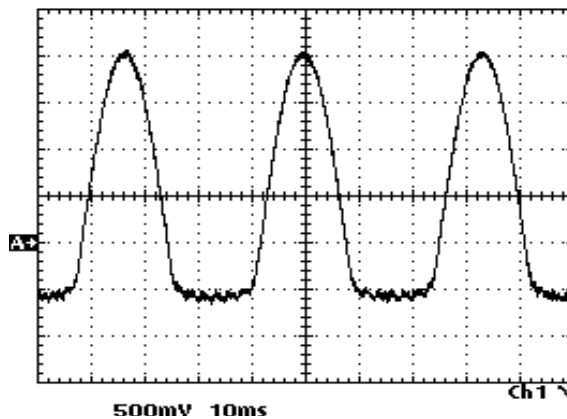
Figure 7-41. Waveform - A8/A24 TP13 Half Wave Rectified 30 Hz FM
