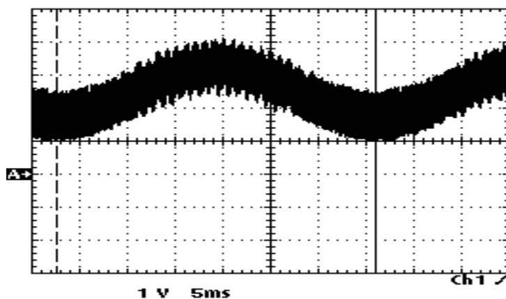
Figure 7-24. Waveform - A12 TP1 Re-configuring for Generator Test of Monitor
