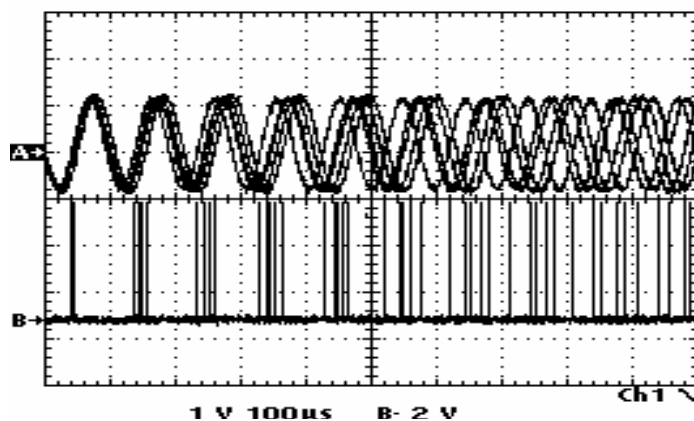
Figure 7-39. Waveform - A8/A24 TP11 and TP12
