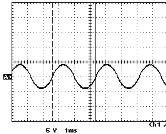
Figure 7-17. Waveform - A7/A23 TP8 360 Hz cos
