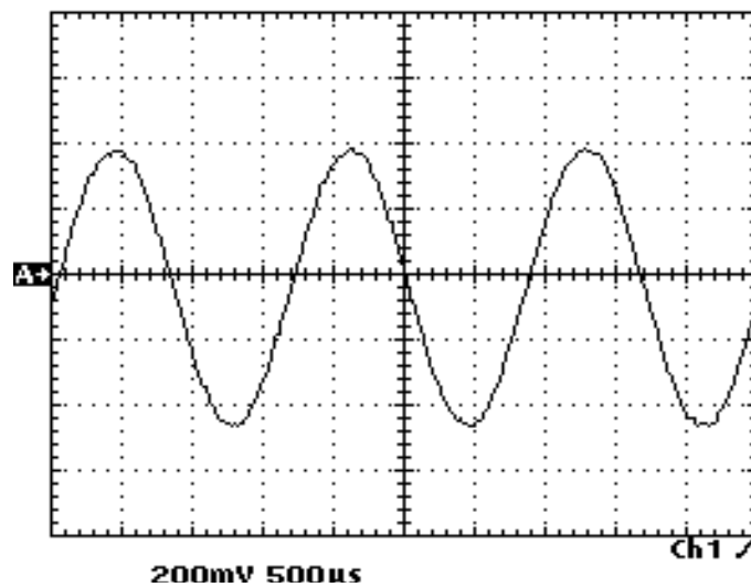
Figure 7-28. Waveform - A8/A24 TP3 600 Hz Voice
