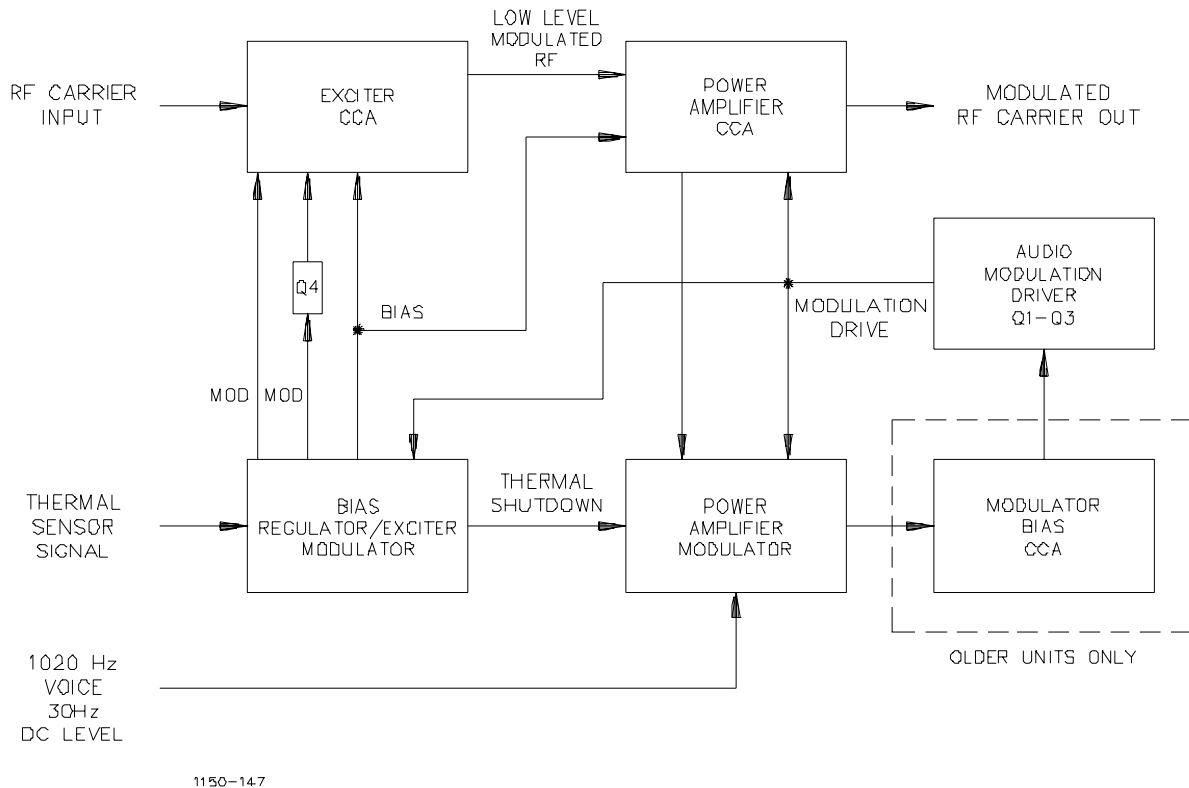
Figure 2-13. CSB Power Amplifier Assembly Block Diagram
