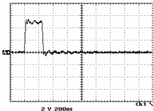
Figure 7-38. Waveform - A8/A24 Monitor CCA TP12
