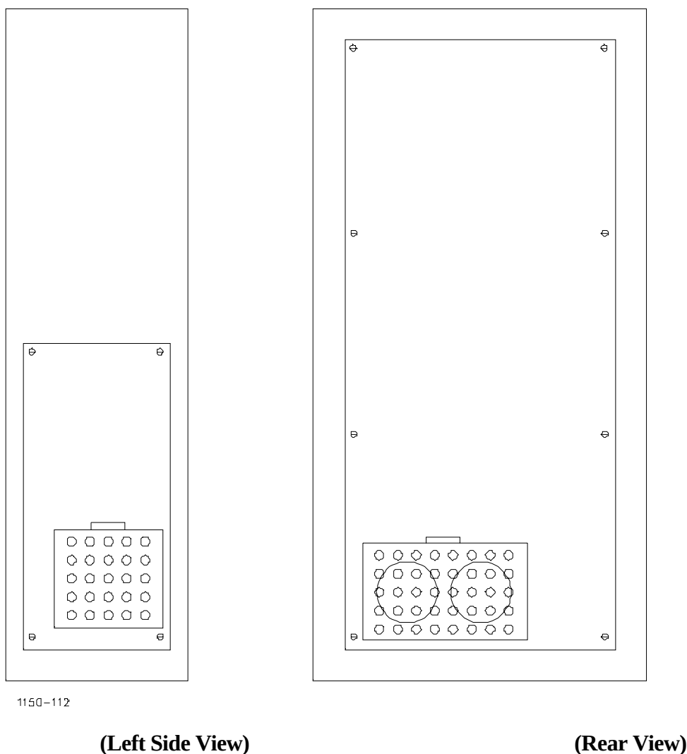
Figure 1-3. DVOR Cabinet
