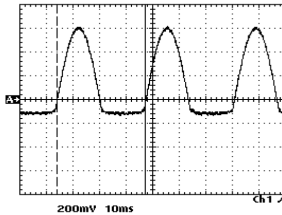
Figure 7-36. Waveform - A8/A24 TP6 Half Wave Rectified
