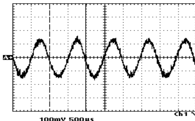
Figure 7-31. Waveform - A8/A24 TP3 Audio Signal Level (ID Only)
