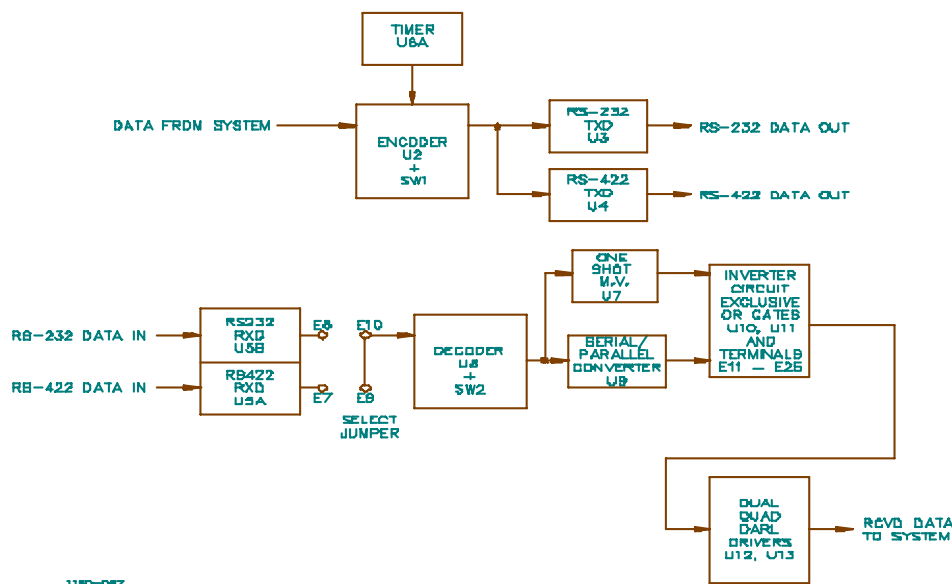
Figure 2-33. RSCU Control Interface CCA (012601), Block Diagram
