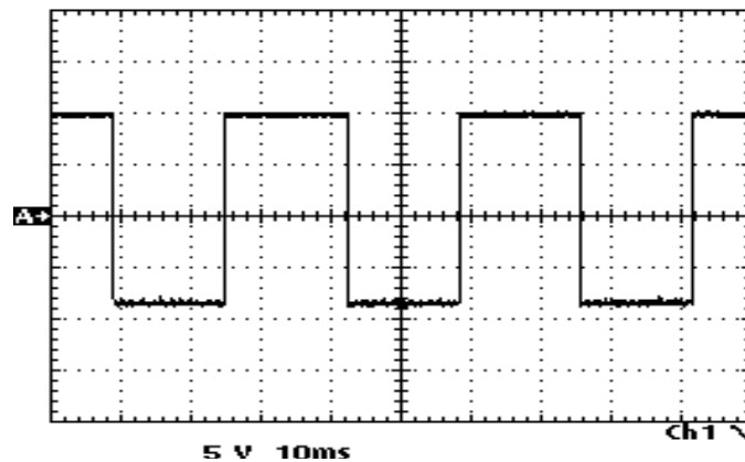
Figure 7-37. Waveform - A8/A24 TP7 30 Hz AM Squared Signal
