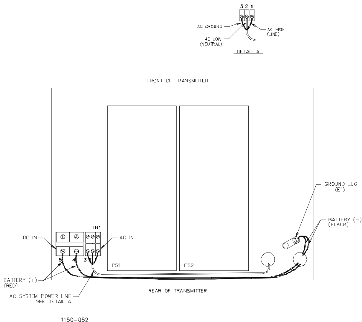
Figure 9-10. AC & DC Interconnect Wiring Diagram
