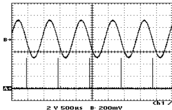
Figure 7-32. Waveform - A8/A24 TP8 Ident Signal Level
