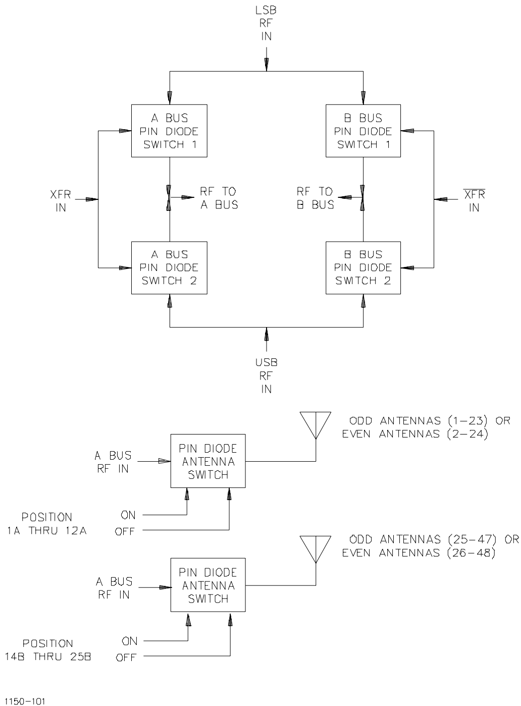
Figure 2-46. Commutator CCA, Block Diagram
