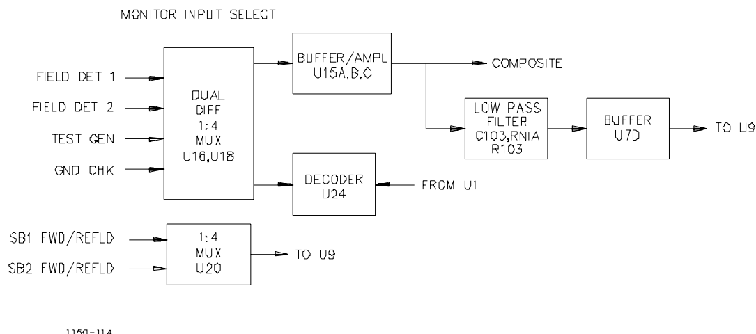
Figure 2-39. Monitor CCA, Block Diagram (sheet 2)
