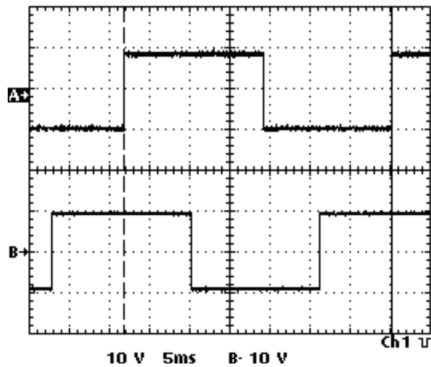
Figure 7-44. Waveform - A8/A24 TP15 and TP7 (90 Degrees)
