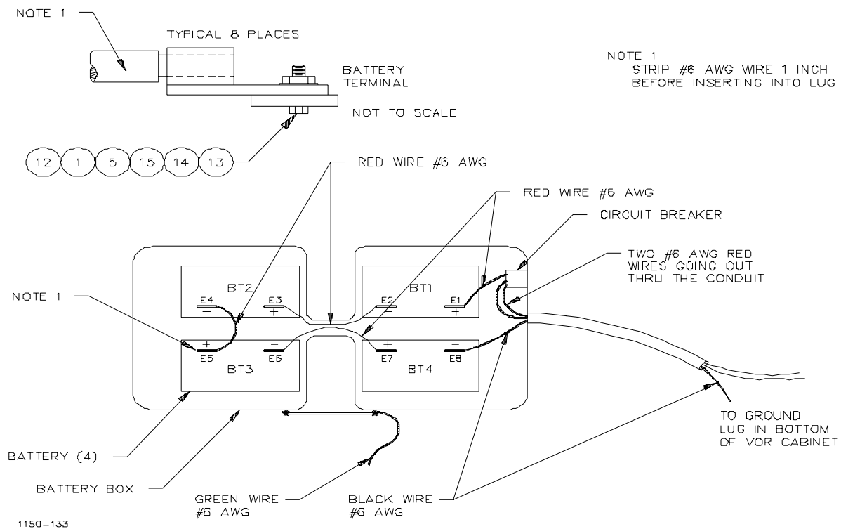
Figure 9-8. Battery Backup Wiring Diagram
