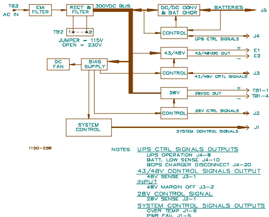
Figure 2-44. Battery Charger Power Subsystem
