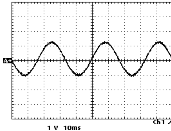
Figure 7-20. Wveform - A7/A23 TP10 30 Hz Reference Signal
