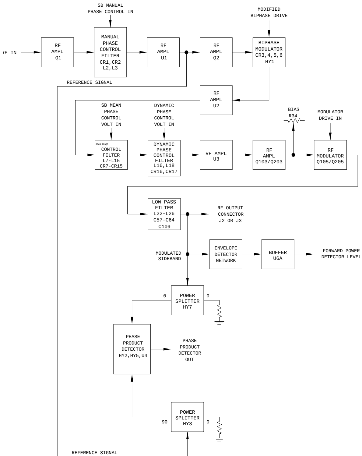
Figure 2-22. Sideband Amplifier CCA Block Diagram
