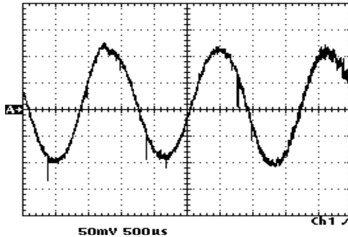
Figure 7-12. Waveform - A7/A23 Signal Generator Output Connected to A38 MIC input
