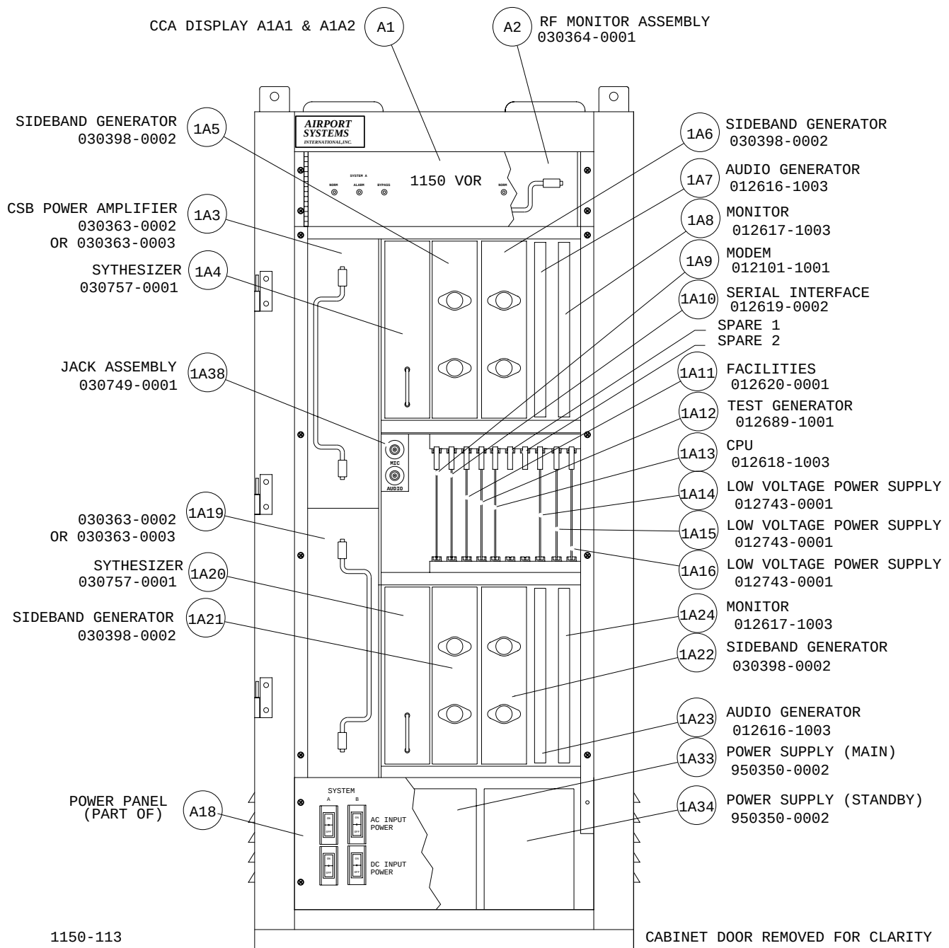
Figure 1-4. Location of Major Assemblies in the Electronics Cabinet (Front View)
