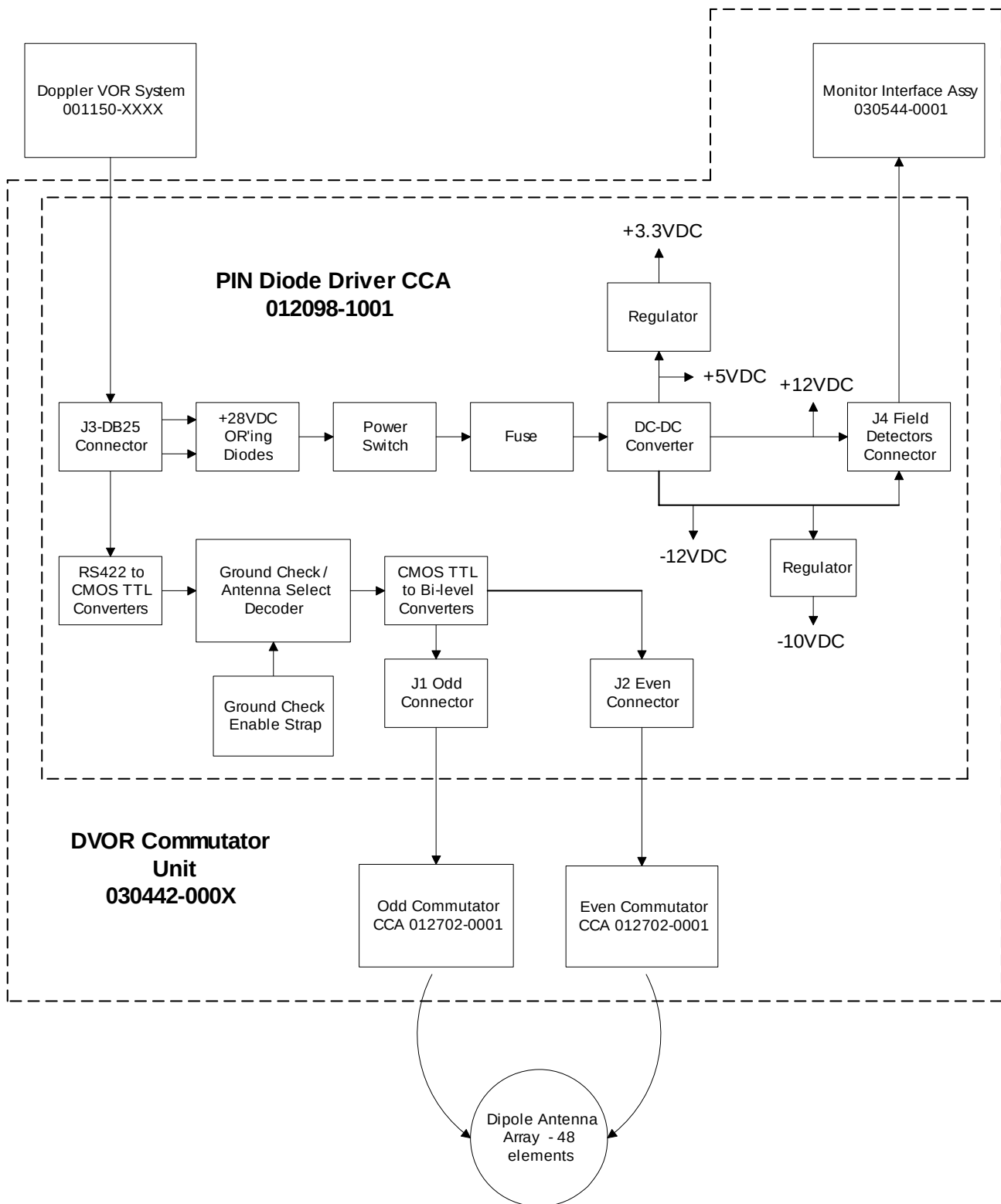
Figure 2-45. Pin Diode Driver CCA, Block Diagram
