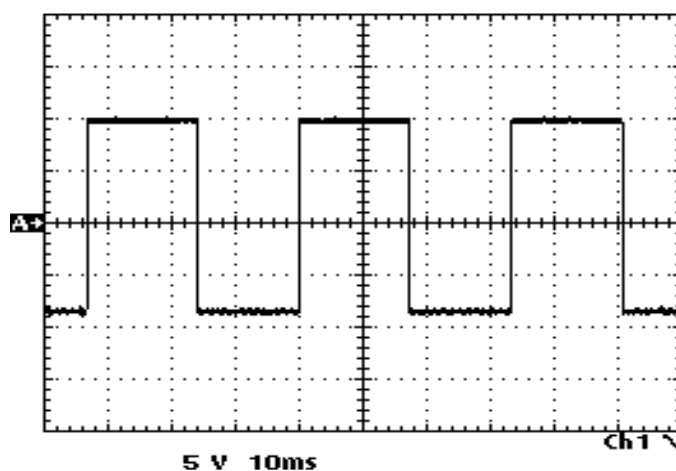
Figure 7-42. Waveform - A8/A24 TP15 30 Hz FM Squared Signal
