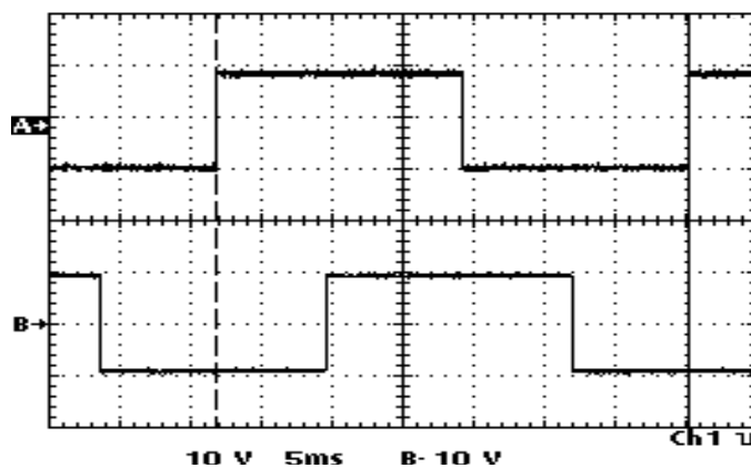
Figure 7-46. Waveform - A8/A24 TP15 and TP7 (270 Degrees)
