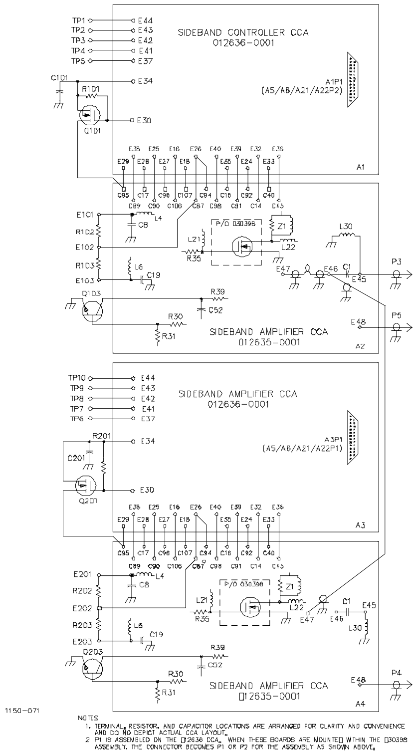
Figure 2-21. Sideband Generator Assembly Interconnect Diagram
