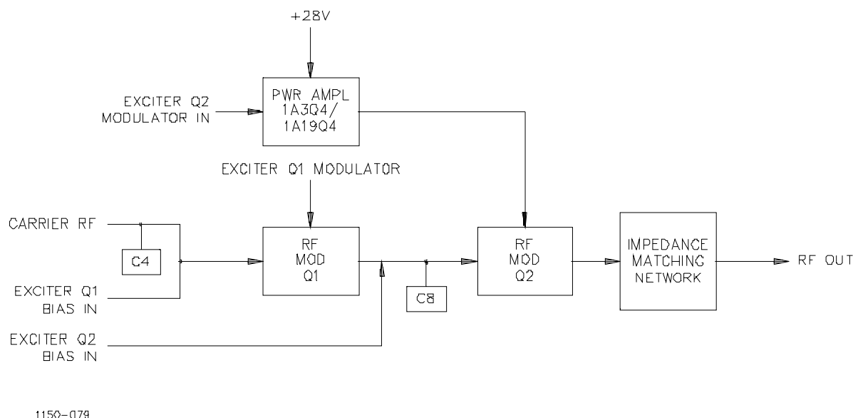
Figure 2-14. Exciter CCA Block Diagram
