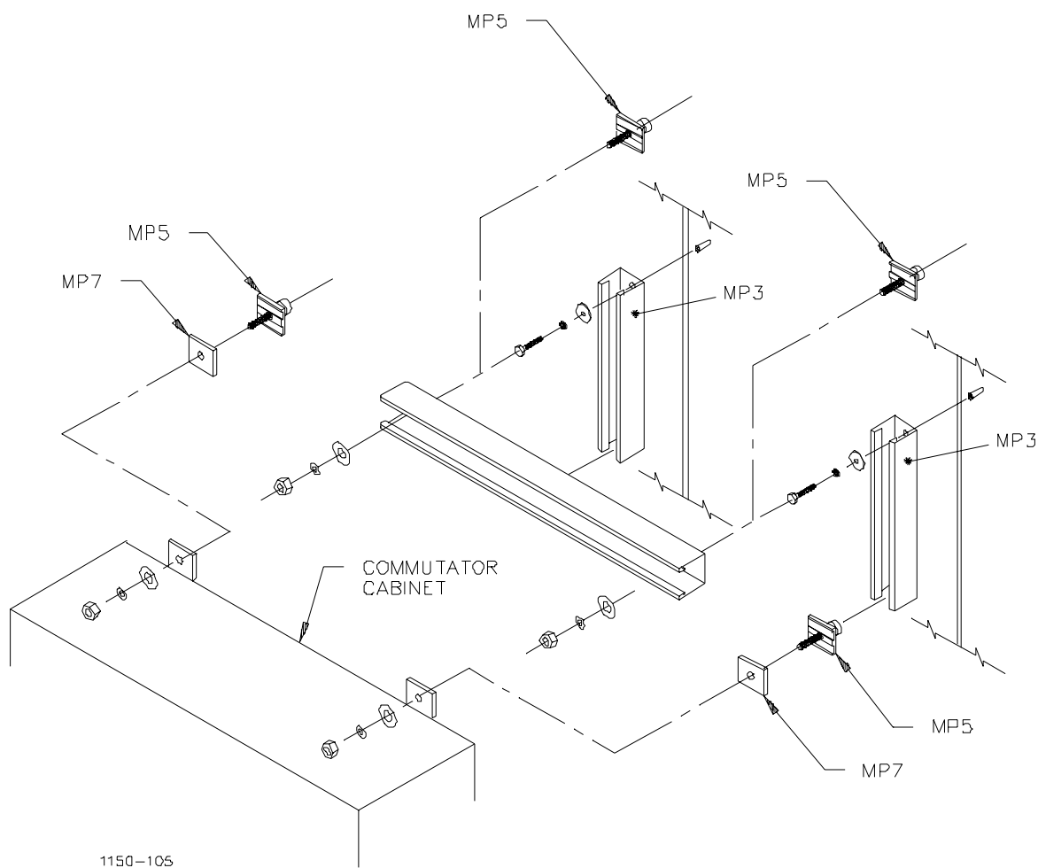
Figure 9-7. Commutator Rack to Shelter Wall Installation Diagram
