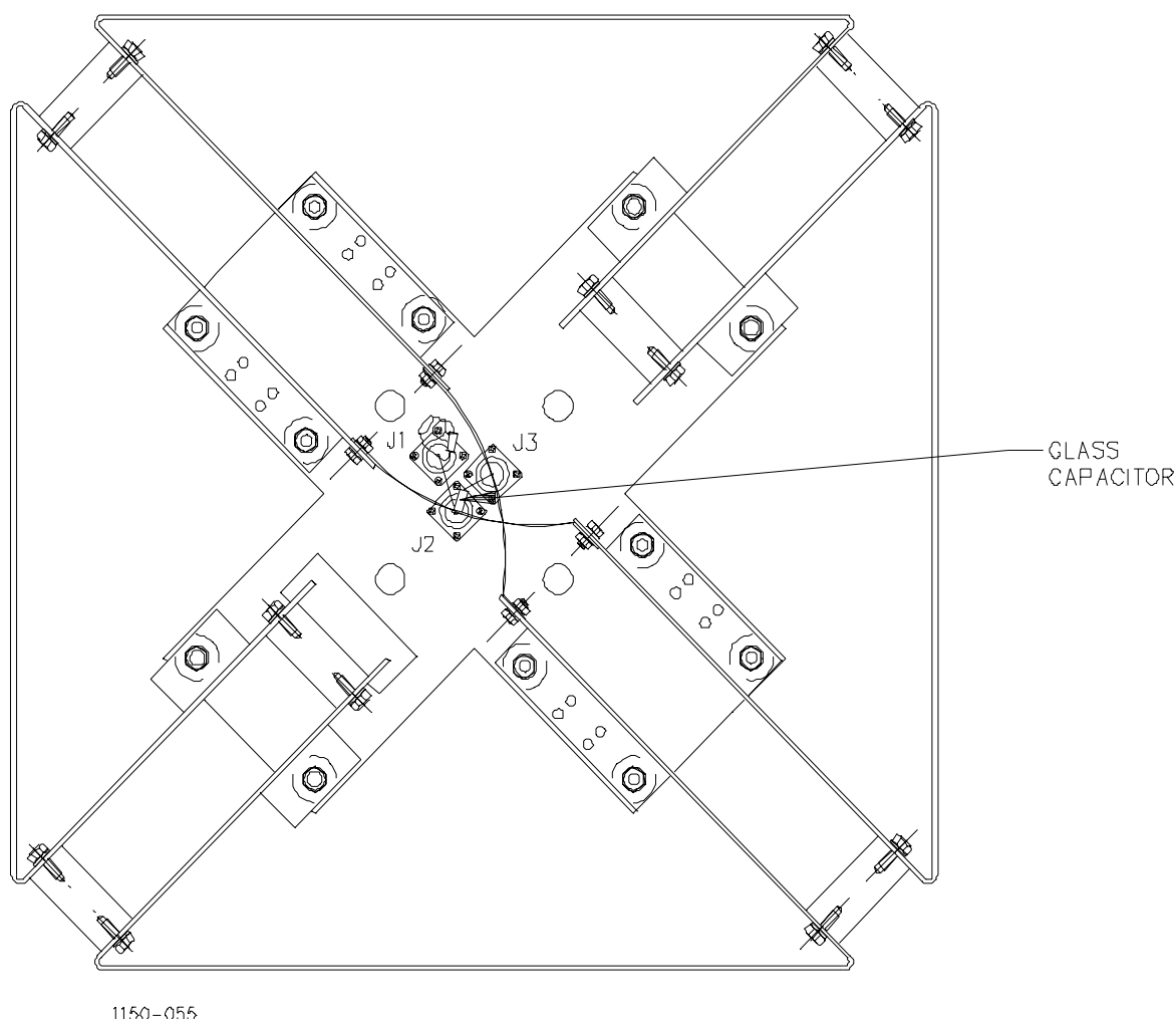
Figure 1-9. Sideband Antenna (Version 2)
