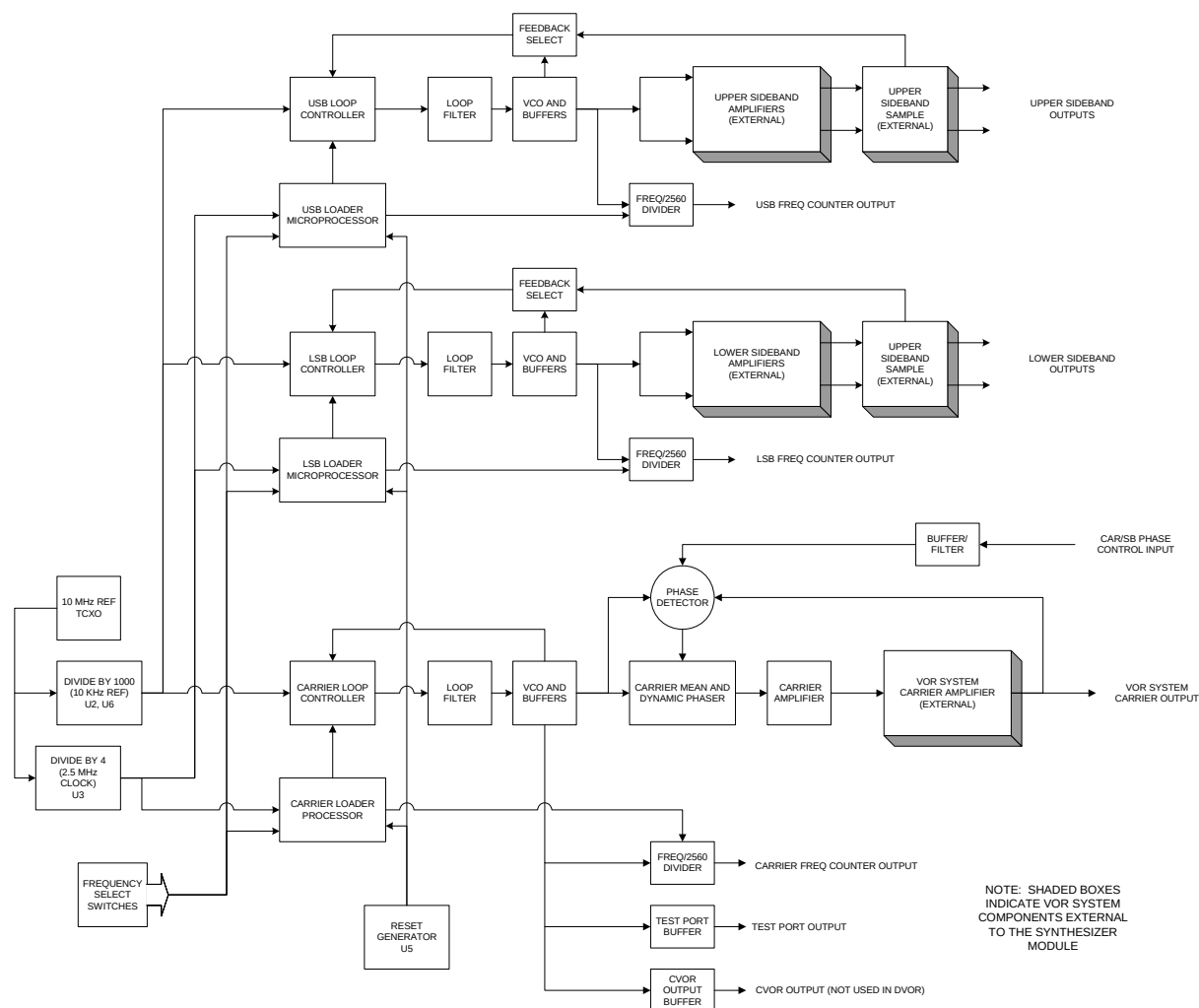
Figure 2-3. DVOR Synthesizer Block Diagram
