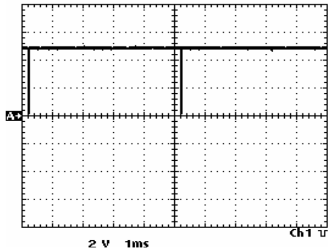
Figure 7-48. Waveform - A8/A24 TP16 200 Hz Clock Pulses (showing time between pulses)
