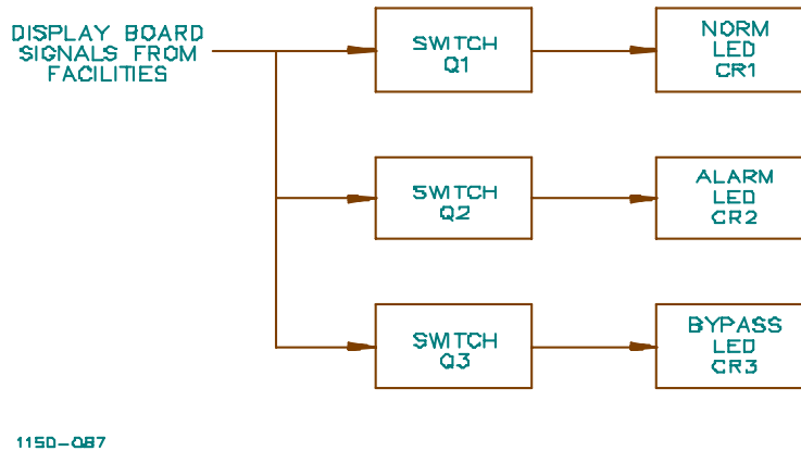
Figure 2-35. Display CCA, Block Diagram
