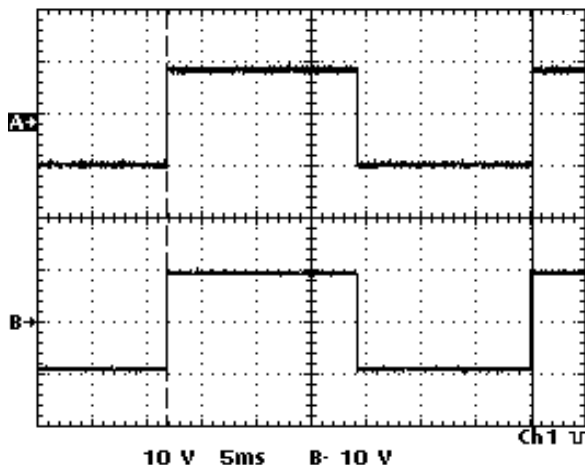
Figure 7-45. Waveform - A8/A24 TP15 and TP7 (180 Degrees)
