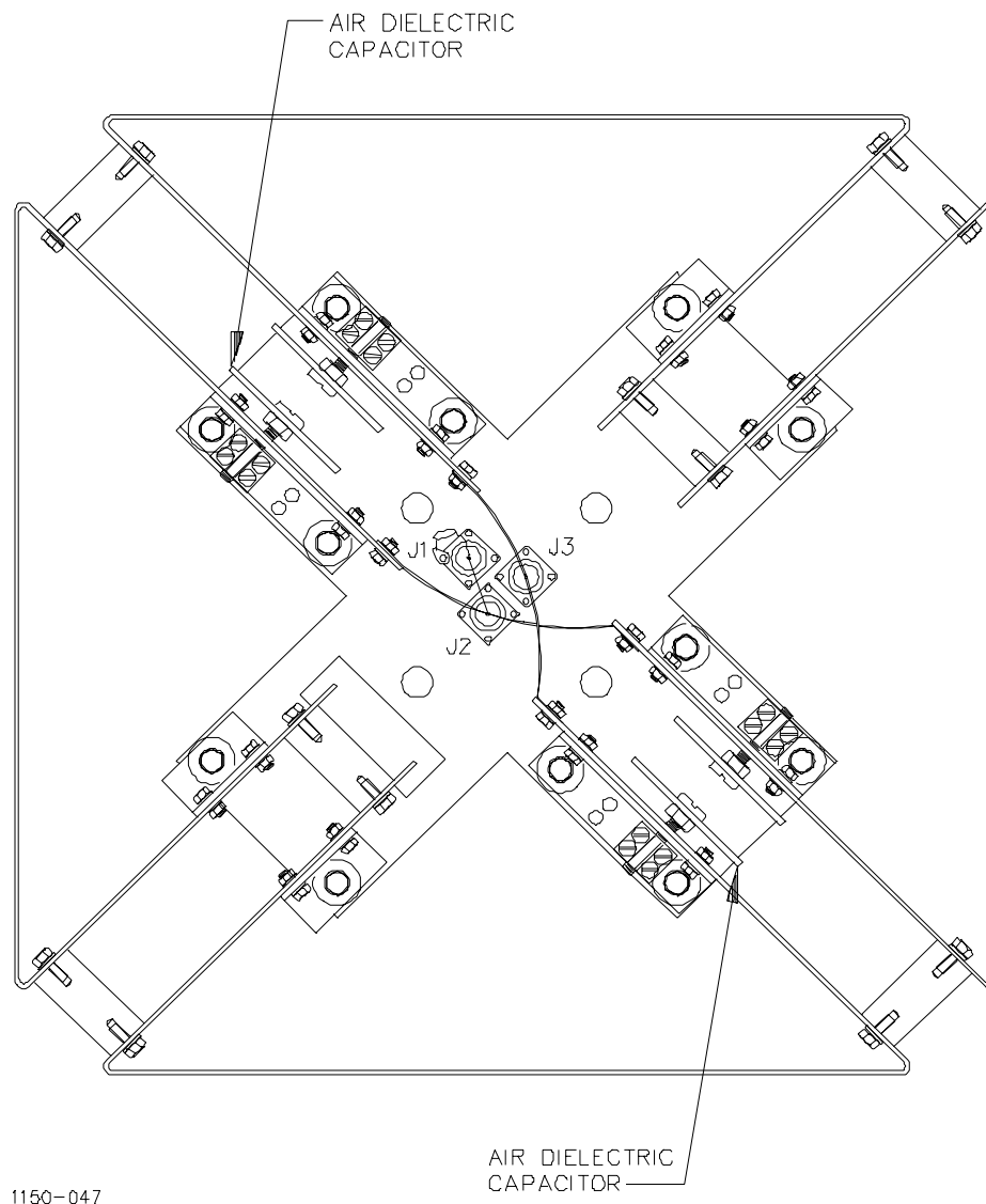
Figure 1-8. Sideband Antenna (Version 1)
