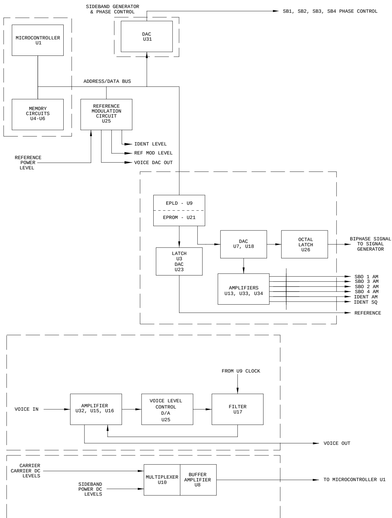
Figure 2-7. Audio Generator CCA, Block Diagram
