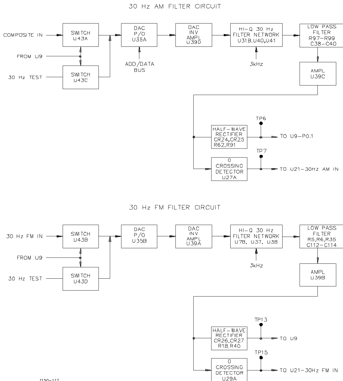
Figure 2-42. Monitor CCA, Block Diagram (sheet 5) (Current Version)
