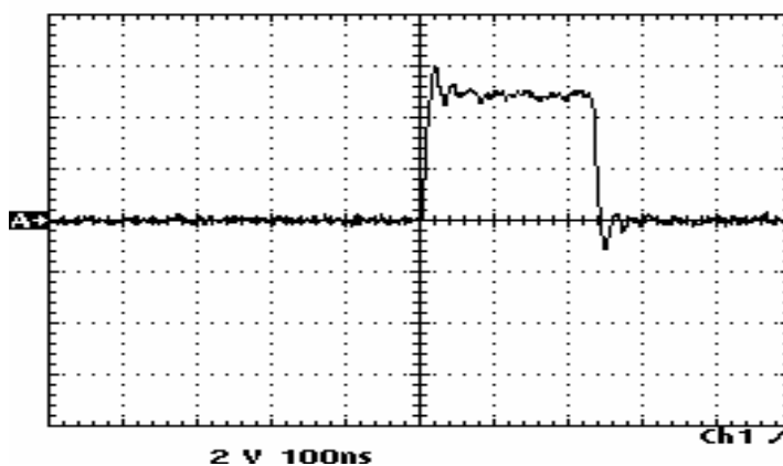
Figure 7-33. Waveform - A8/A24 TP9 ID Square Pulse
