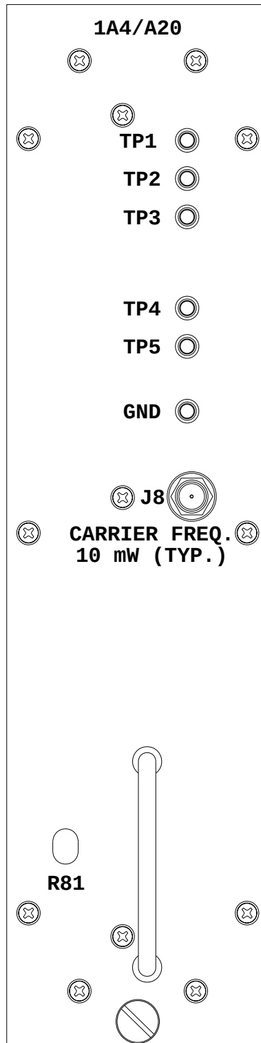
Figure 9-17. Frequency Generator; Front Panel View
