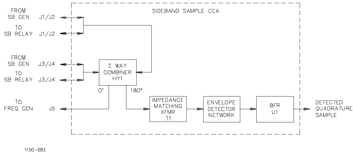
Figure 2-24. Sideband Sample CCA Block Diagram
