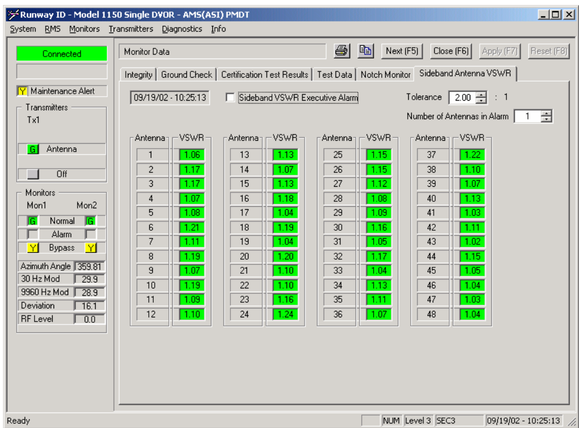
Figure 3-27. Sideband Antenna VSWR
