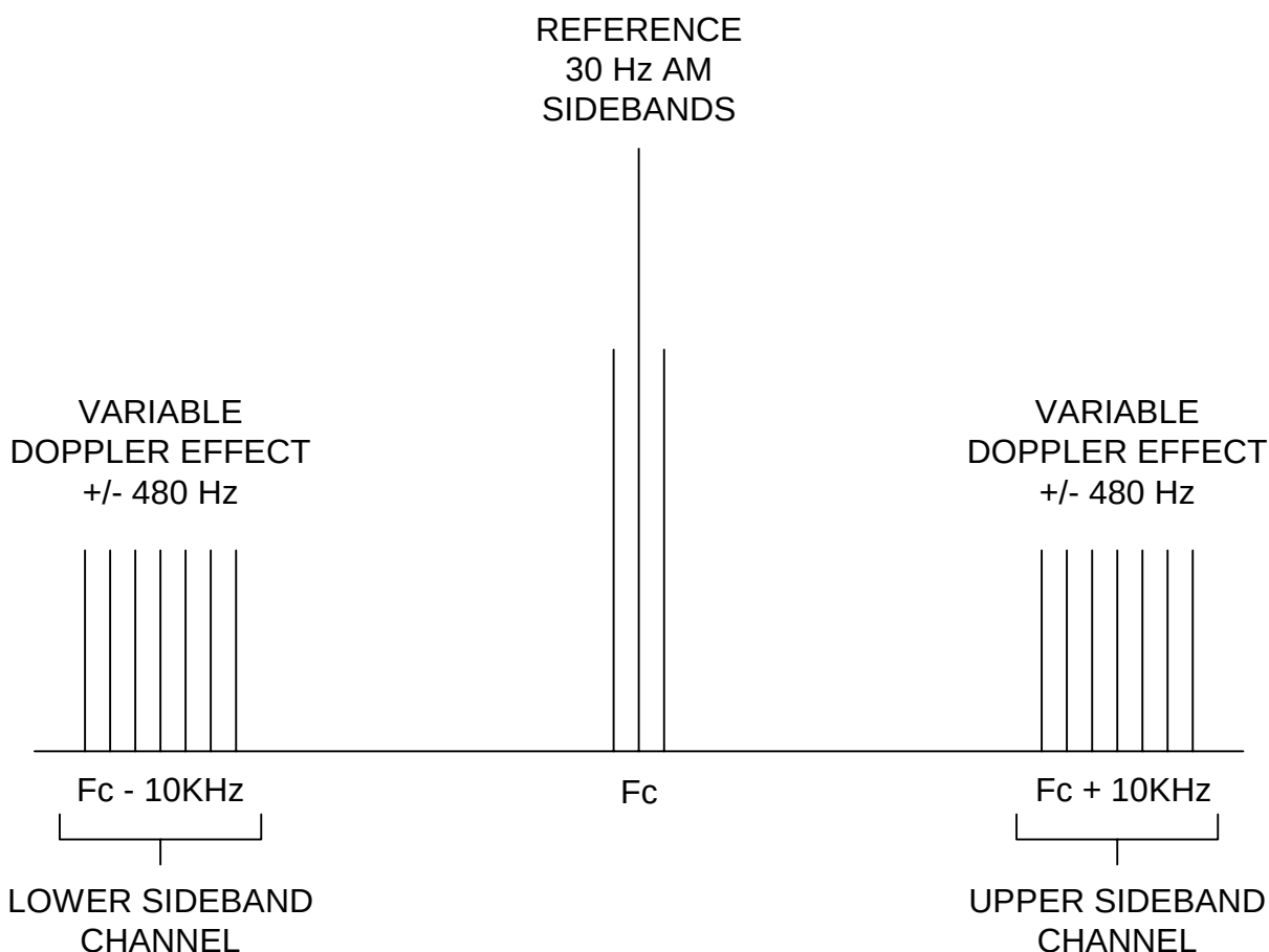
Figure 2-1. RF Spectrum of a Doppler VOR
