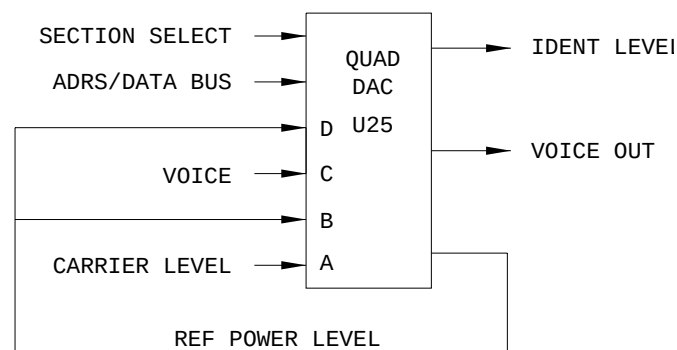
Figure 2-10. Audio Generator CCA Block Diagram (Reference Modulation Circuit).
