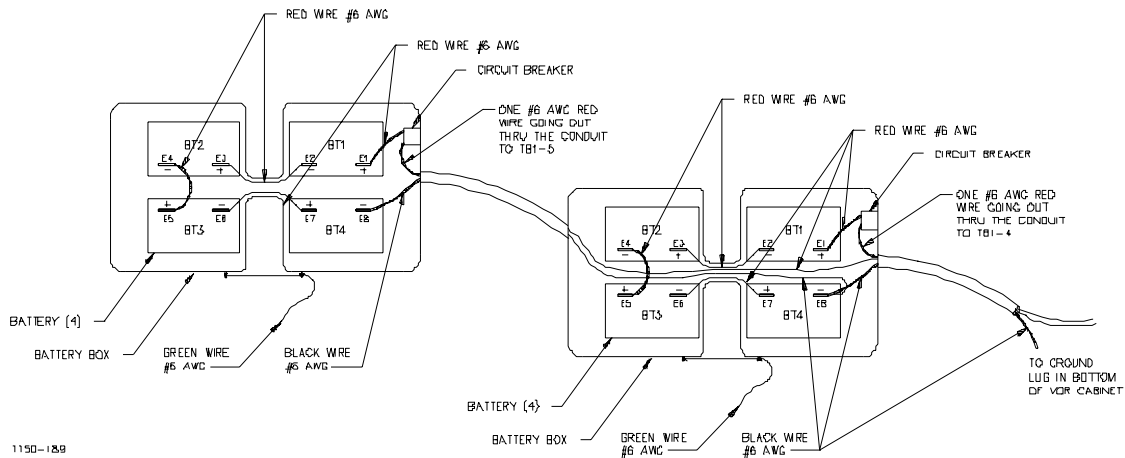
Figure 9-9. Dual Battery Backup Wiring Diagram
