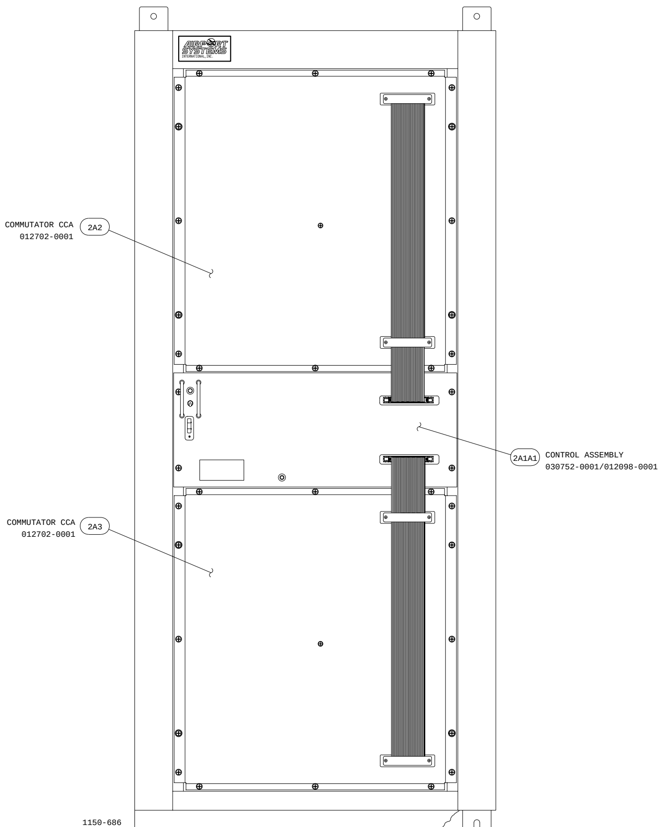
Figure 1-5. Commutator Rack
