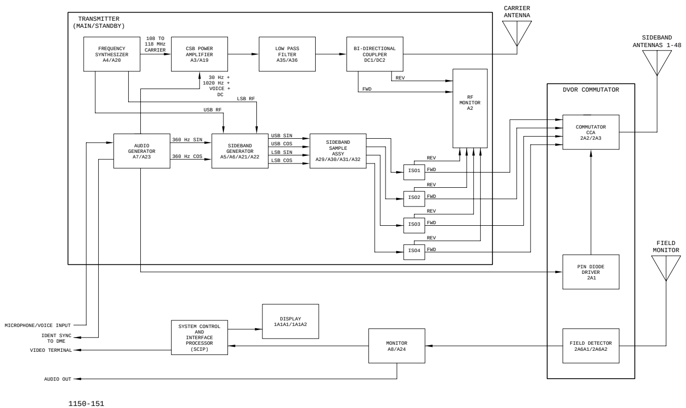
Figure 2-2. Simplified DVOR System Block Diagram
