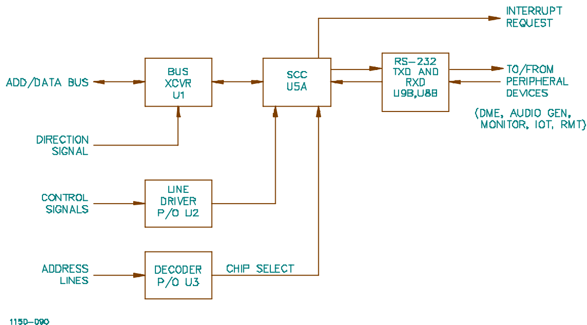
Figure 2-30. Serial Interface CCA, Block Diagram (Typical SCC Communications Circuit)
