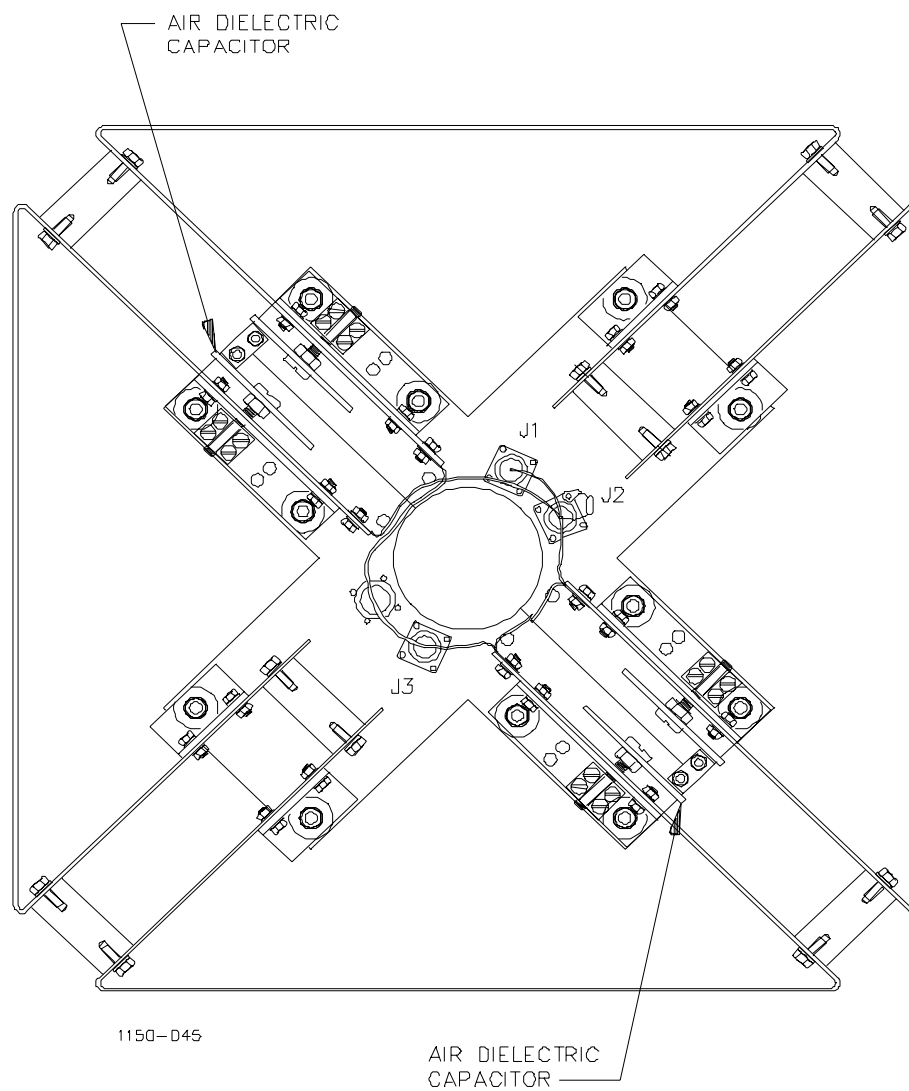
Figure 1-6. Carrier Antenna (Version 1)
