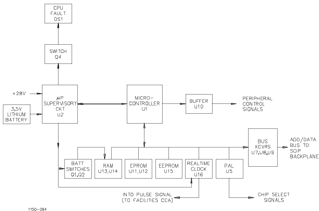
Figure 2-28. CPU CCA Block Diagram
