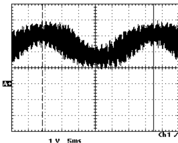
Figure 7-30. Waveform - A8/A24 TP5 Composite Signal
