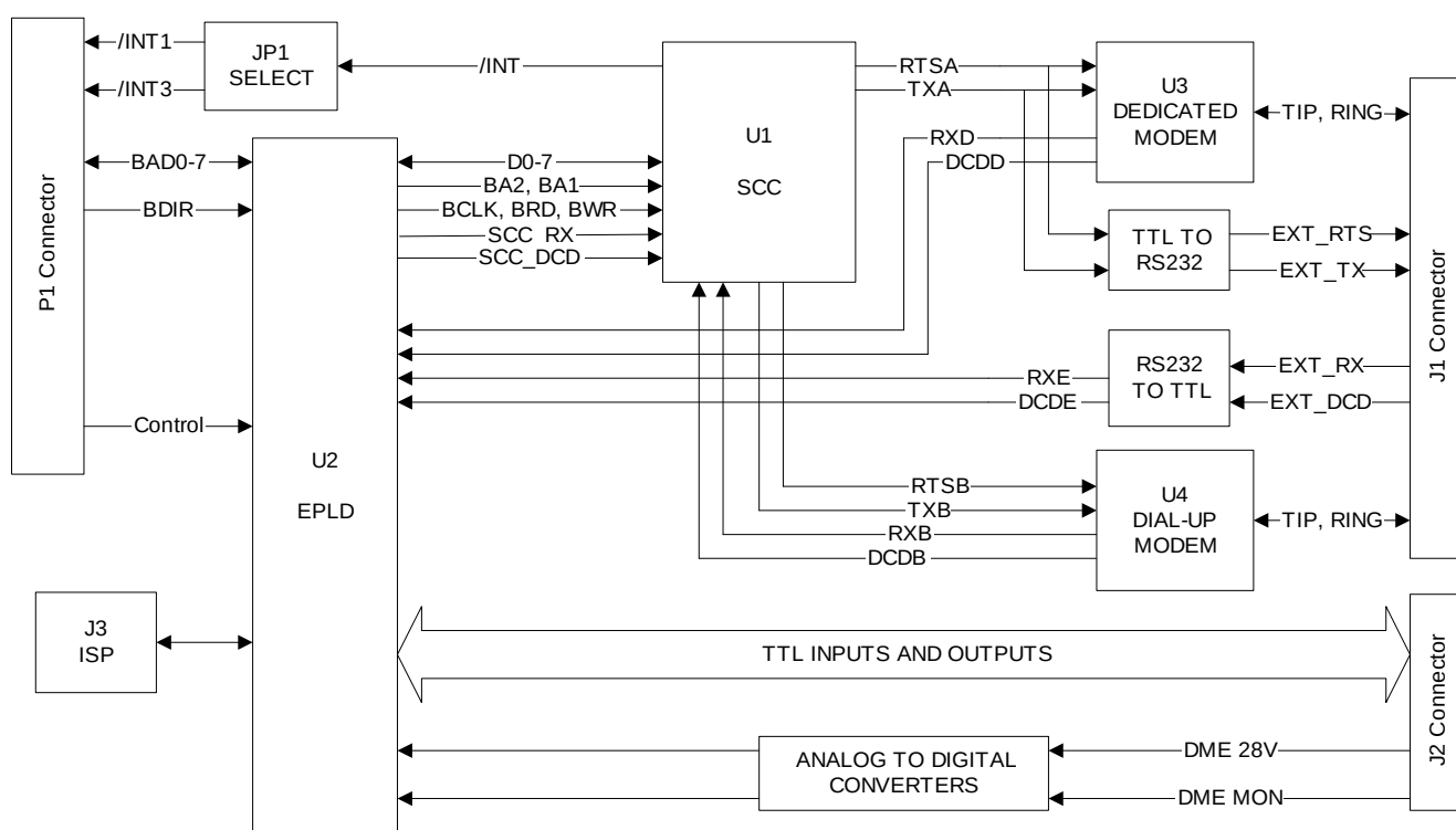
Figure 2-32. Modem CCA (012101-1001), Block Diagram
