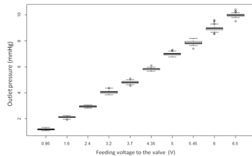
Figure 2. Box and whisker plot of the outlet pressure (tube exit) according to the feeding voltage of the valve (V) for the 700 \mu m internal diameter tube
