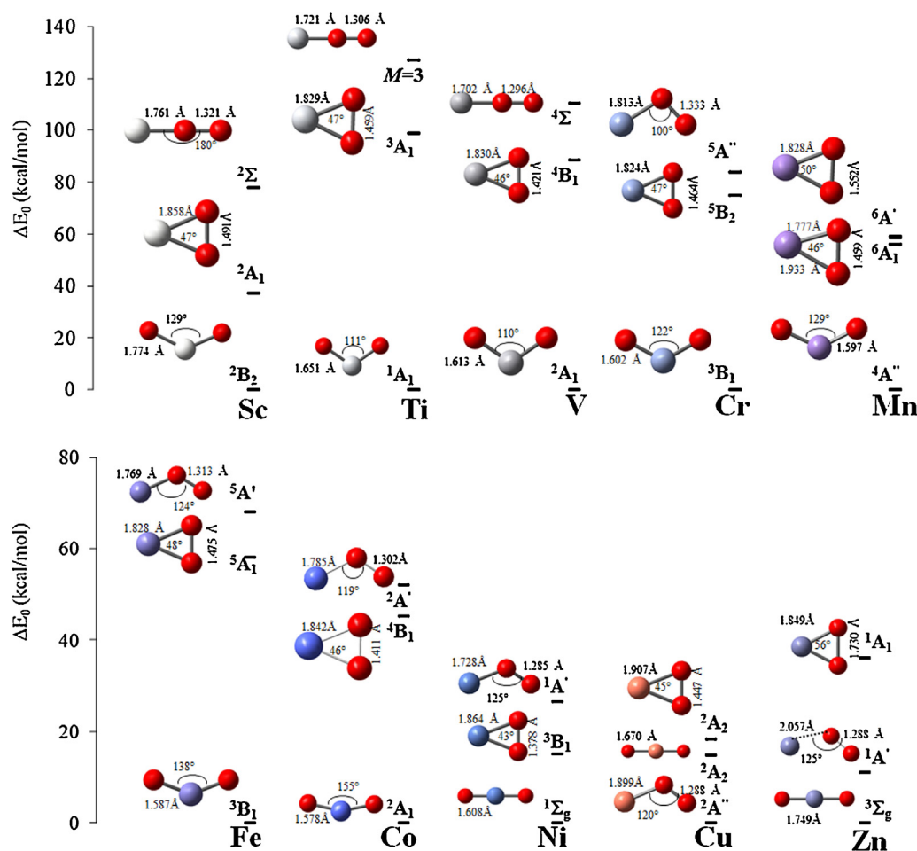
Figure 2. Energies (in kcal/mol) of transition metal peroxide and superoxide complexes given with respect to the total energy of the ground state of each particular dioxide.
