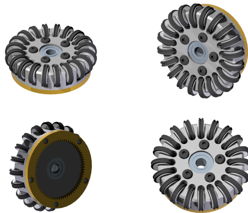
Fig. 3. Different views for the computational model of the new wheels of the STOx's 3 rd generation. Its diameter is larger than that of previous generations and it contains 5 more rollers
