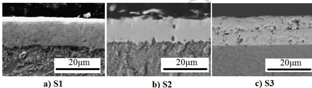
Figure 2. SEM micrographs of the coatings produced on AISI D2 steel. a) S1 b) S2 and c) S3.
