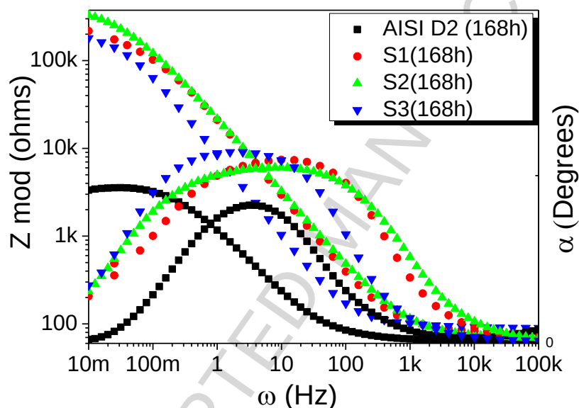
Figure 8. Bode plots of EIS spectra of AISI D2 (uncoated), S1, S2 and S3.
