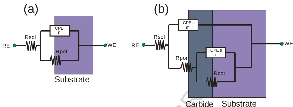
Figure 9. Equivalent circuits: (a) Bare steel and (b) coated steels.
