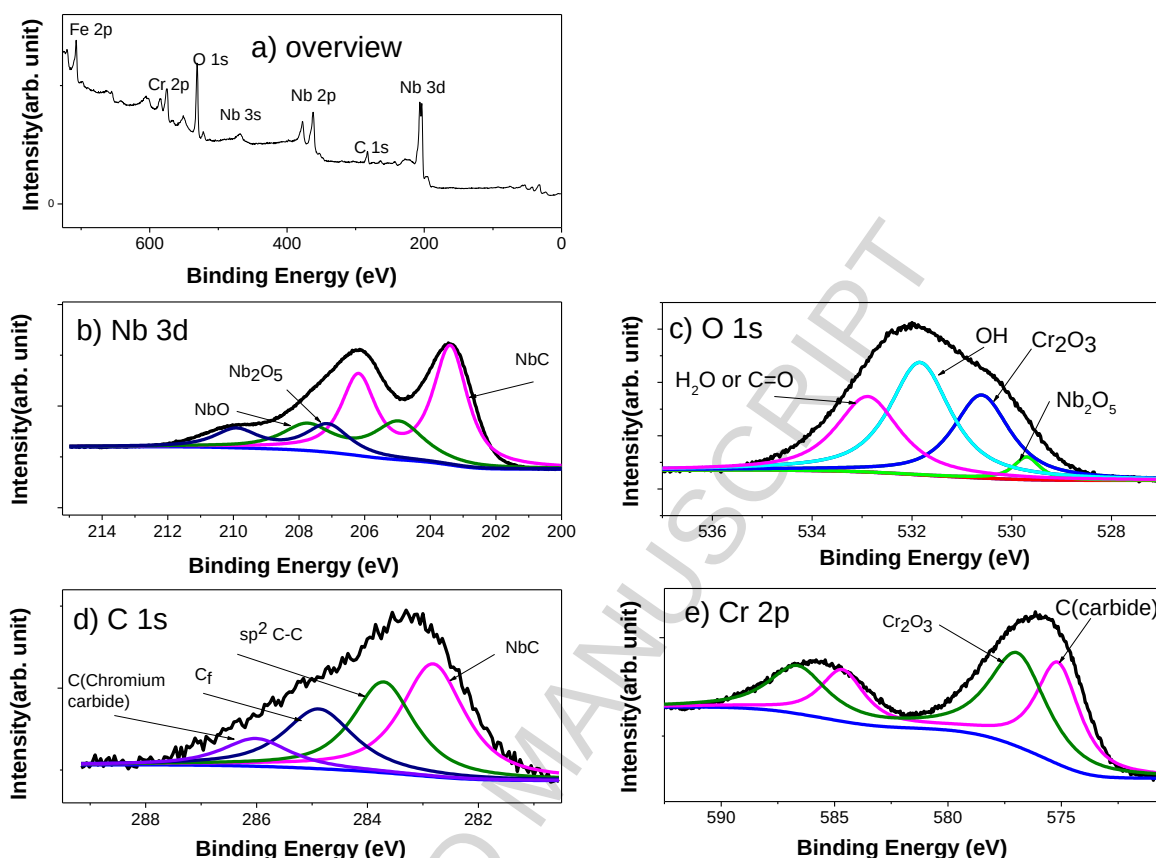
Fig. 4. XPS spectra for sample S3 a) Overview b) Nb 3d c) O 1s, d) C 1s spectra and e) Cr 2p spectra.
