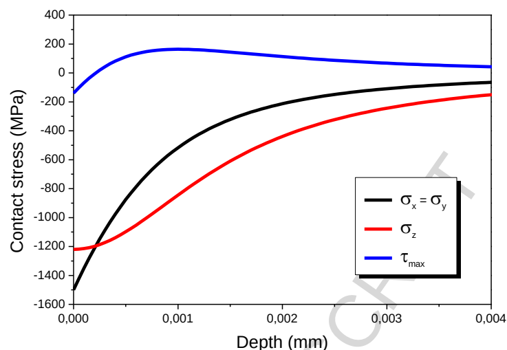
Figure 1. Shear stress distribution in the Niobium-Chromium carbide coating on AISI D2 produced through TRD
