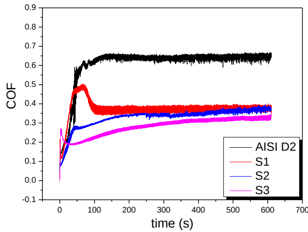
Fig. 5. Friction coefficient measurement of the coatings produced.
