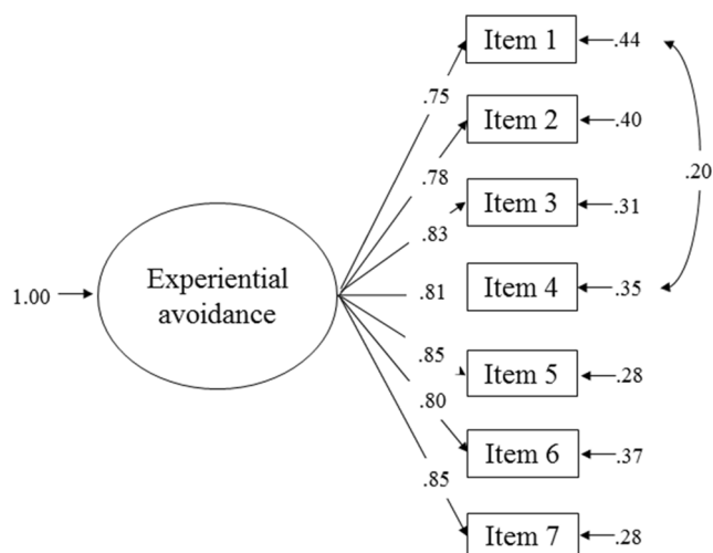
Fig. 1 Standardized solution for the one-factor model with correlated measurement errors between items 1 and 4 in the overall sample
