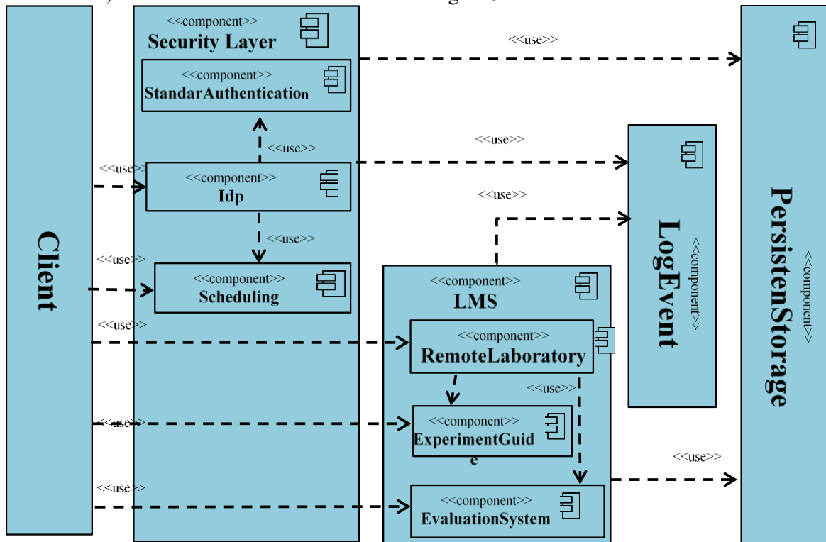
Figure 5. LMS architecture with non-functional requirements.
